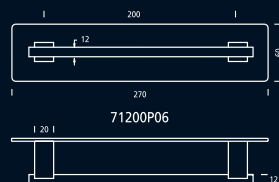
71200P06 Tirador 200mm sobre placa de 60x270mm. Pull handle, 200mm, on 60x270mm plate. Tirant ou 200mm, sur plaque (60x270mm).
