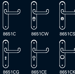
8651C Manilla sobre placa de 225x45mm. Handle on 225x45mm plate. Béquille sur plaque (225x45mm).
