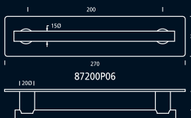
87200P06 Tirador 200mm sobre placa de 60x270mm. Pull handle, 200mm, on 60x270mm plate. Tirant ou 200mm, sur plaque (60x270mm).
